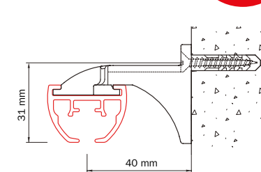
Wall mounting with bracket 6051
