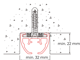
Concealed mounting, for example, in channel with bracket 6055-3100-N-040 when creating bends: cut the channel on the basis of the track supplied by Qurails
