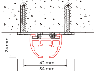
Ceiling mounting with bracket 6055-1000
