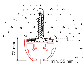
Ceiling mounting with ceiling mounting clamp 6050
