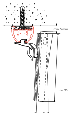
5600 heading with projection glider 6010
