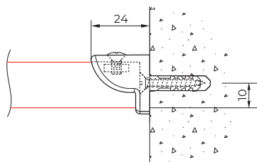
wall mounting 4200 with wall bracket 24249
