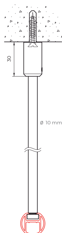
ceiling mounting with 4255
