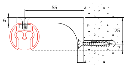
wall mounting 5100 with wall bracket 5140
