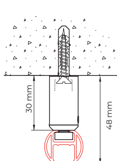
ceiling mounting 4200 with suspenson hanger 4254
