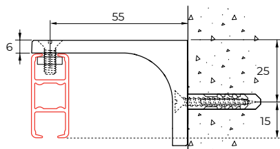
wall mounting 4100 with wall bracket 4140
