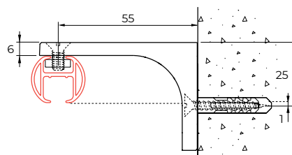
wall mounting 4200 with wall bracket 5140
