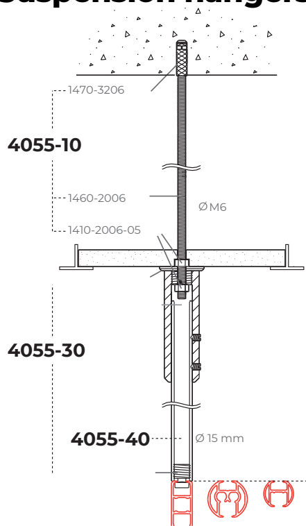
- ceiling mounting 4100, 5100 or 4200: threaded rod set 4055-10, suspension hanger tube 4055-40 and with mounting set 4055-30
