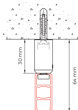
ceiling mounting 4100 with suspenson hanger 4254
